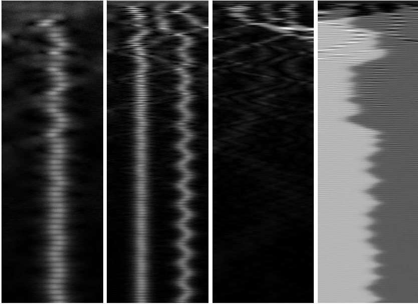
Fig. 8. Focusing of random initial data. Grey levels code the absolute value of u along the chain horizontally, and time proceeds downwards. Left to right, the initial data is u_0 = 0.9, 2.0, 2.5, and 3.0 . Superimposed noise variance is 0.1 . Damping is set to zero. Sequence corresponds to AAV1 from position 200 to 400 (see text).
