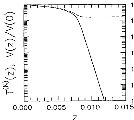
FIG. 2. The transmission coefficient T^{(N)} (solid line) and the function V(z)/V(0) (dashed line) when initial conditions are N(0) = 0.625 , V(0) = 0.5 [ \alpha(0) = 1.25 ].
