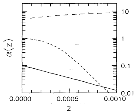
FIG. 4. The parameter \alpha(z) for different choices of \alpha(0) . V(0) = 0.1 in all three cases. Solid line, \alpha(0) = 0.1 [ N(0) = 0.01 ]; short-dashed line, \alpha(0) = 1 [ N(0) = 0.1 ]; long-dashed line, \alpha(0) = 5 [ N(0) = 0.5 ].
